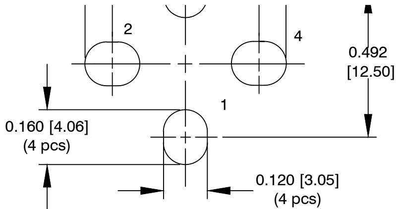
MOUTING HOLES PATTERN
